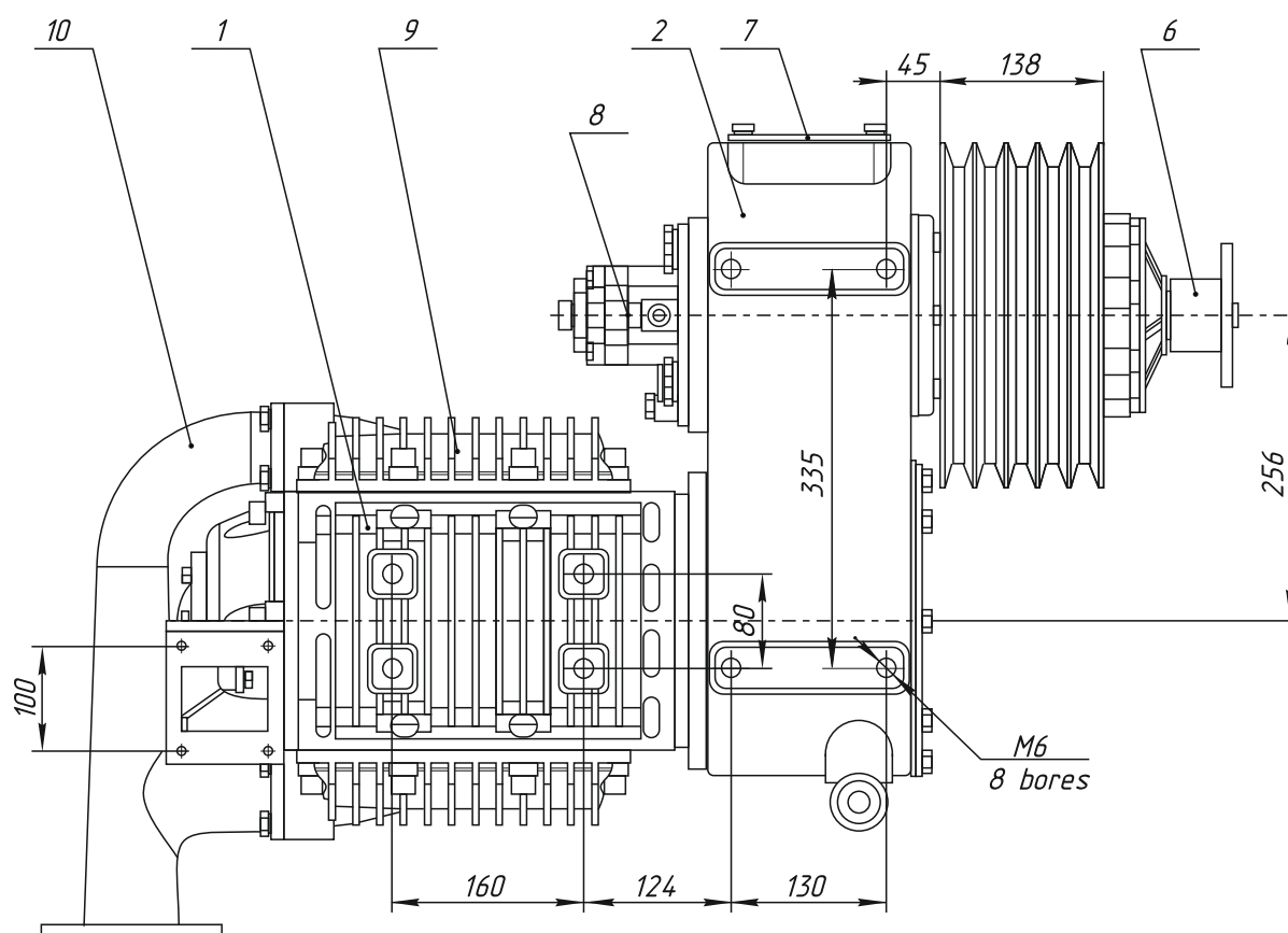
Pendulum oil-free compressor KM-10-2R1.Riflon. Dimentions.
